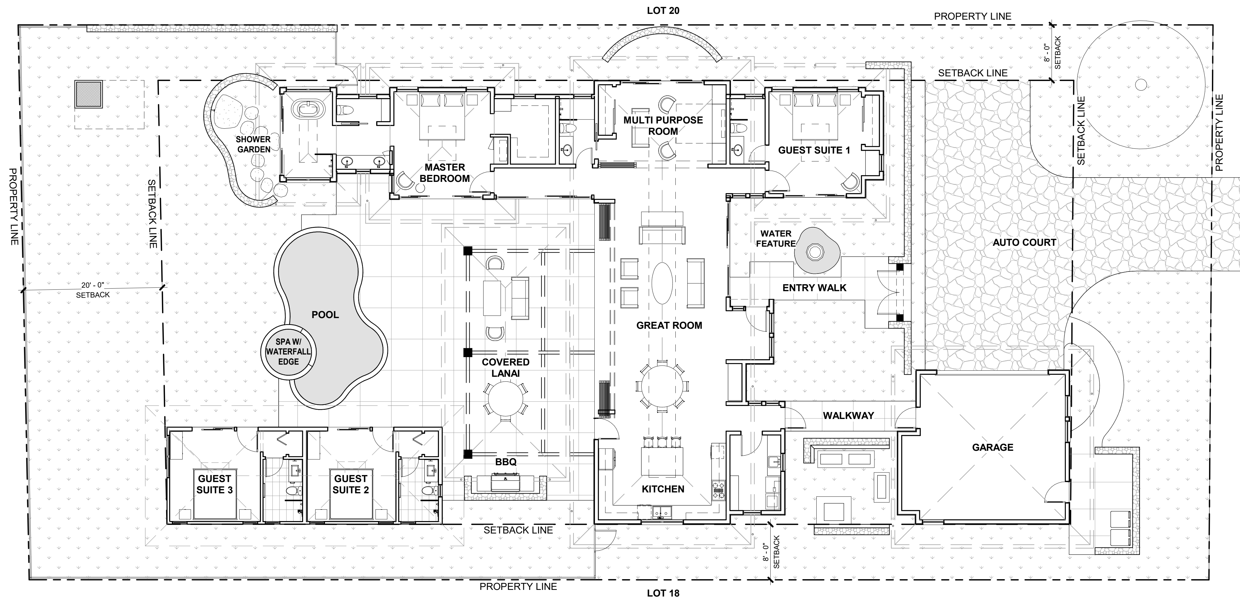
1 A1.2 LOT 19 SITE PLAN SCALE: 1/8" = 1'-0"
