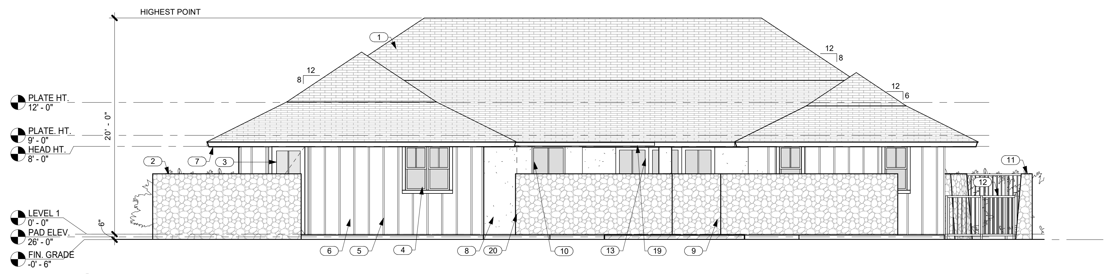
2 NORTH ELEVATION A3.0 SCALE: 3/16" = 1'-0"
