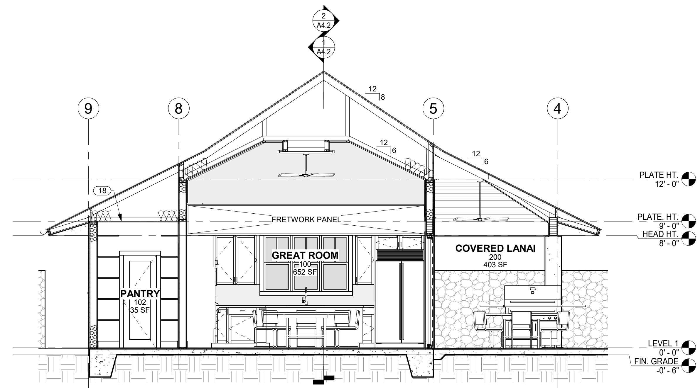
2 SECTION THRU GREAT ROOM, COVERED LANAI AND PANTRY LOOKING NORTH
