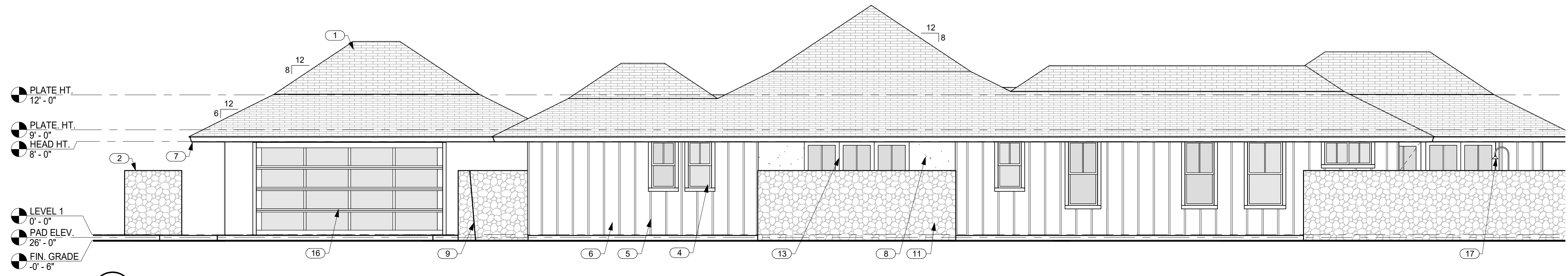
4 WEST ELEVATION A3.0 SCALE: 3/16" = 1'-0"
