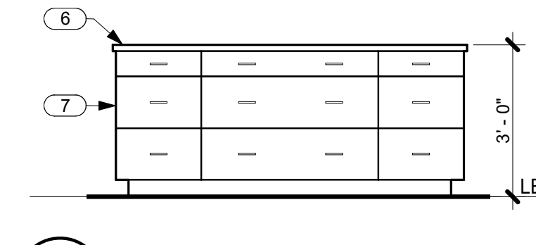
3 NORTH SIDE OF KITCHEN ISLAND A7.0 SCALE: 3/8" = 1'-0"
