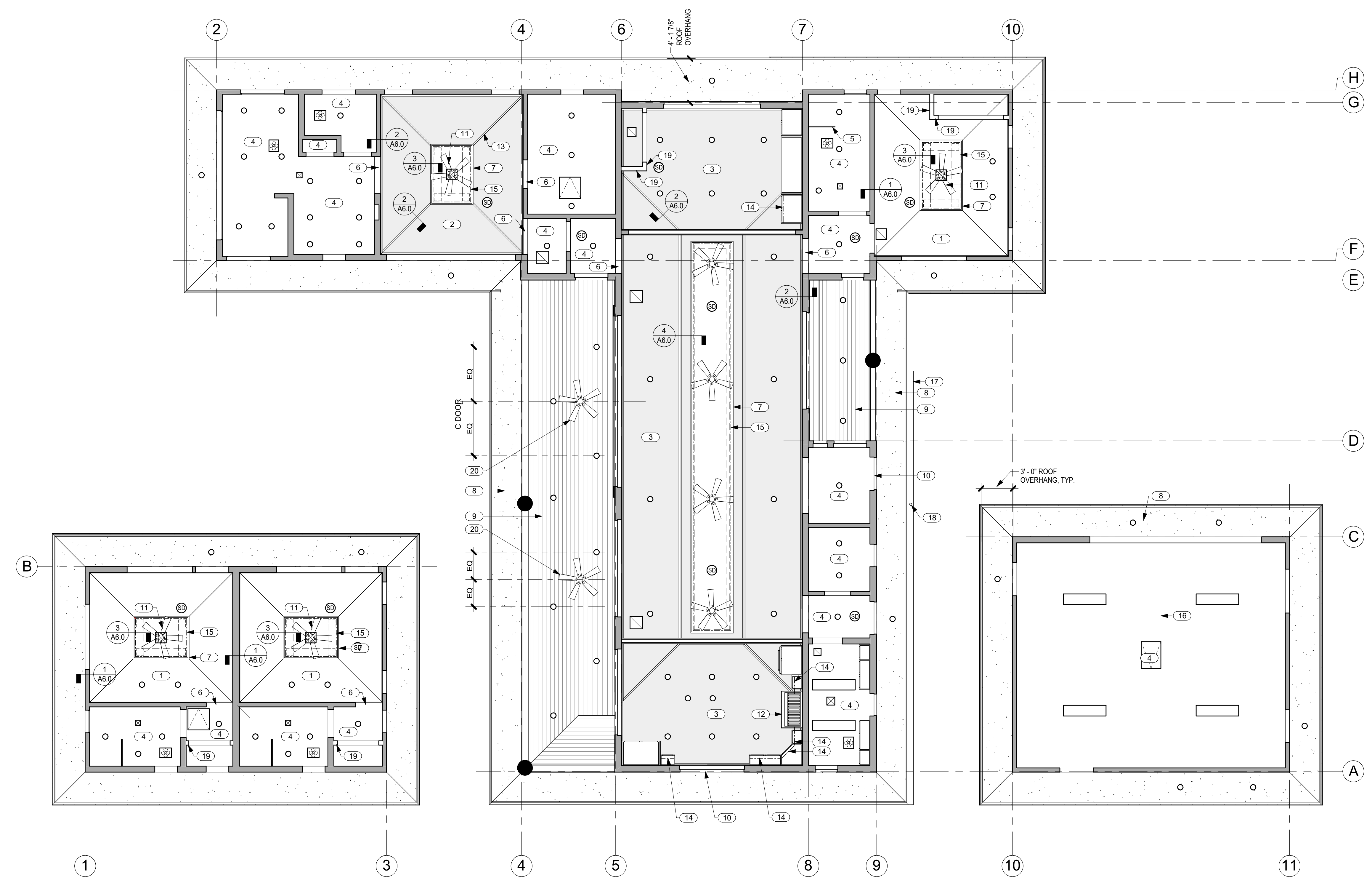
1 REFLECTED CEILING PLAN A2.4 SCALE: 3/16" = 1'-0"
