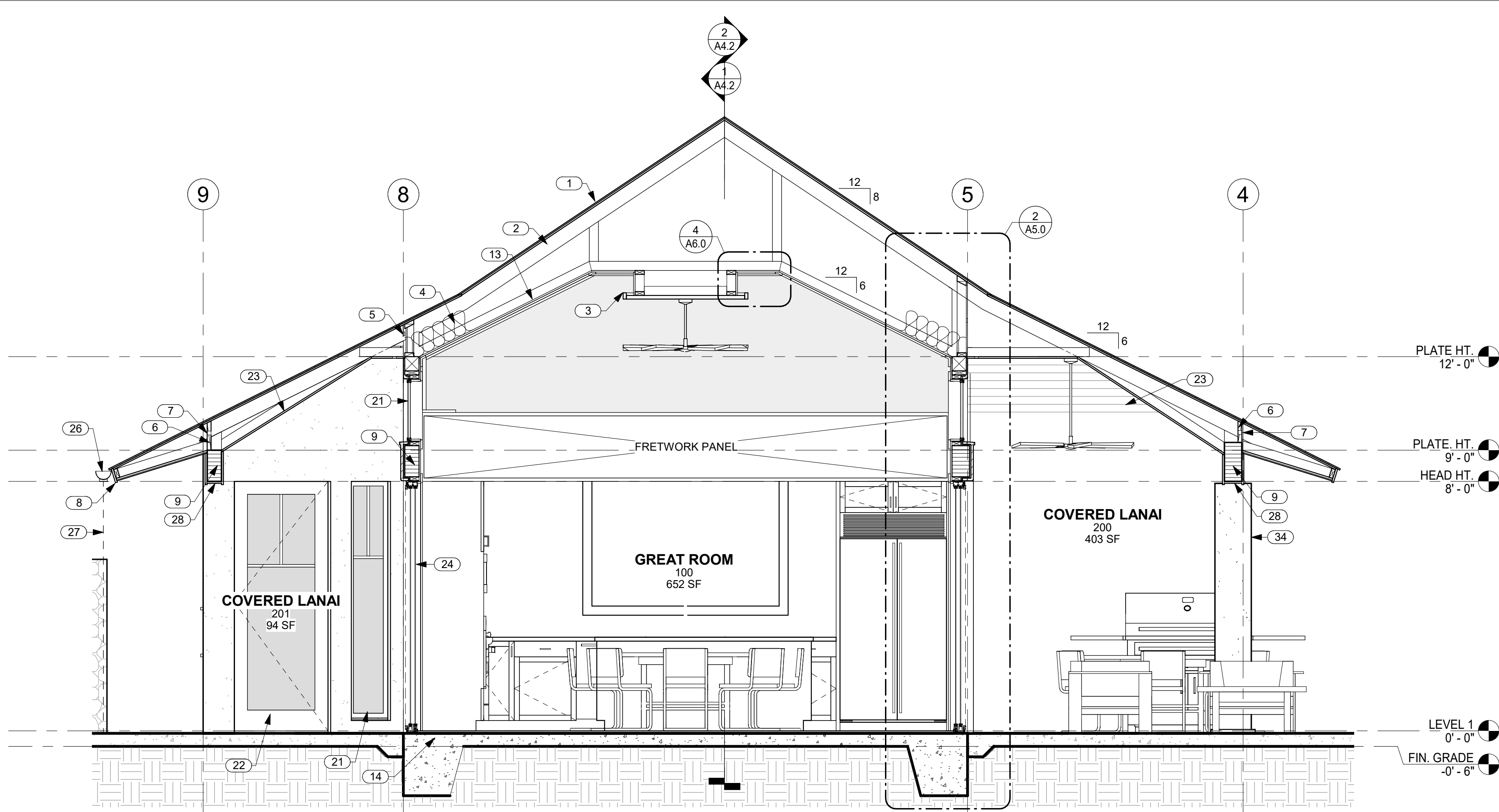
1 SECTION THRU GREAT ROOM AND COVERED LANAIS LOOKING NORTH
