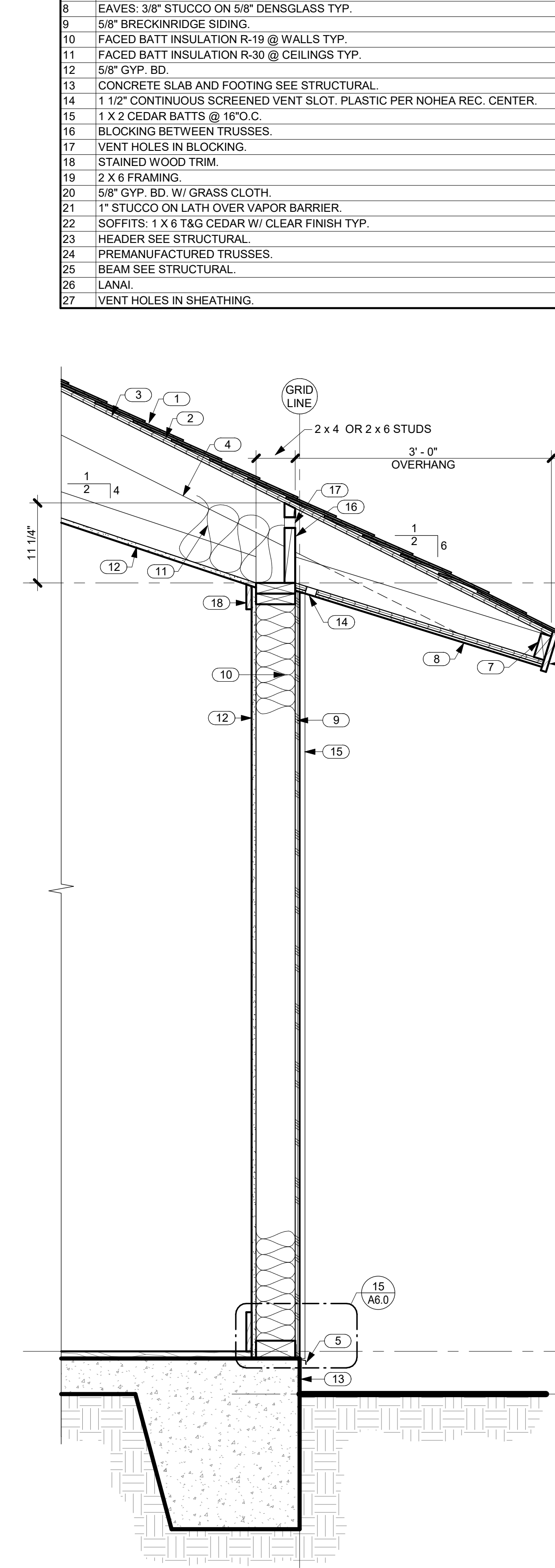
3 TYP. WALL SECTION @ GUEST SUITE BEDROOMS A5.0 SCALE: 1" = 1'-0"
