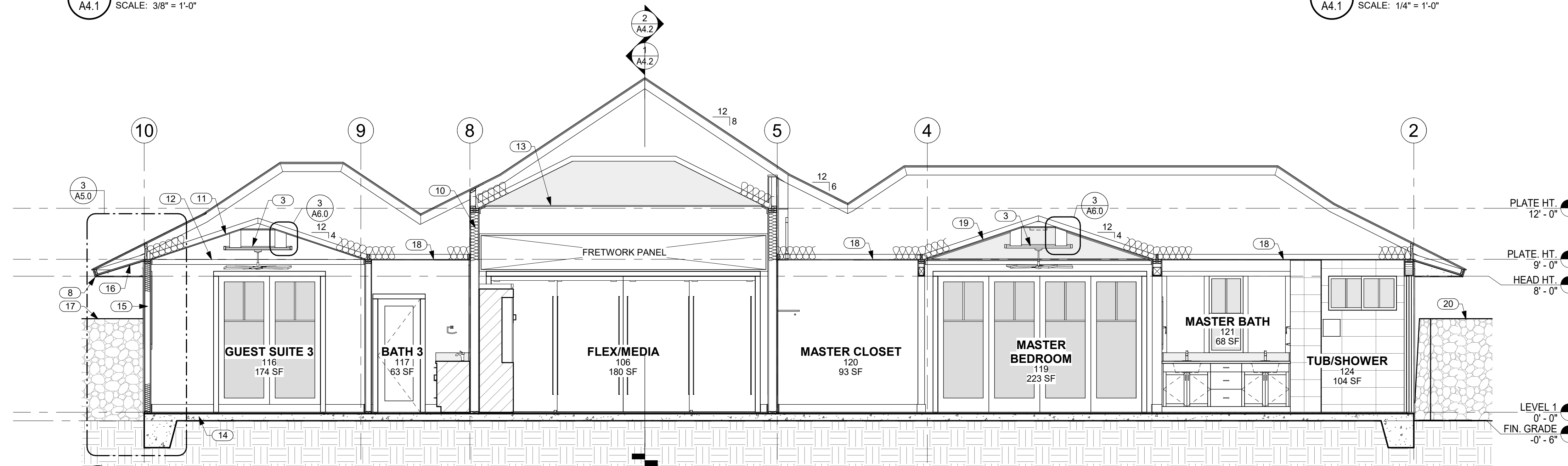
3 BUILDING SECTION LOOKING NORTH
