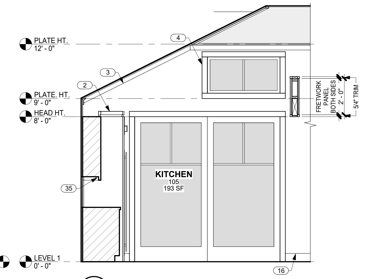
4 WEST WALL KITCHEN 105 A7.0 SCALE: 3/8" = 1'-0"
