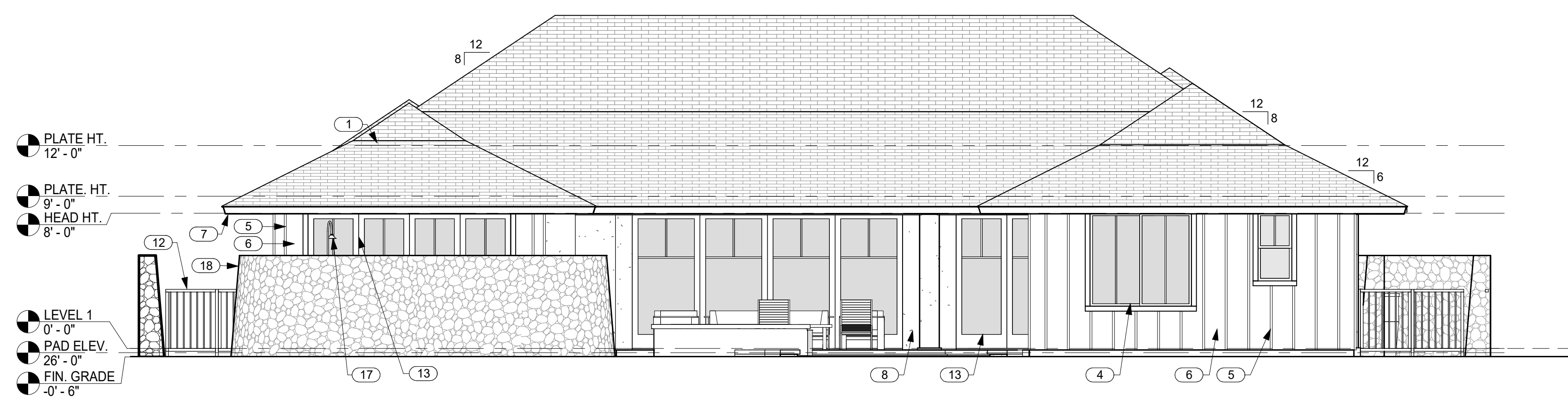
5 SOUTH ELEVATION A3.0 SCALE: 3/16" = 1'-0"
