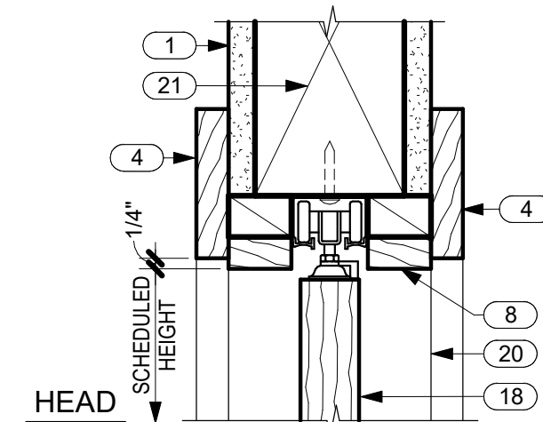
5 TYP. BI-FOLD DOOR TRACK A6.1 SCALE: 3" = 1'-0"
