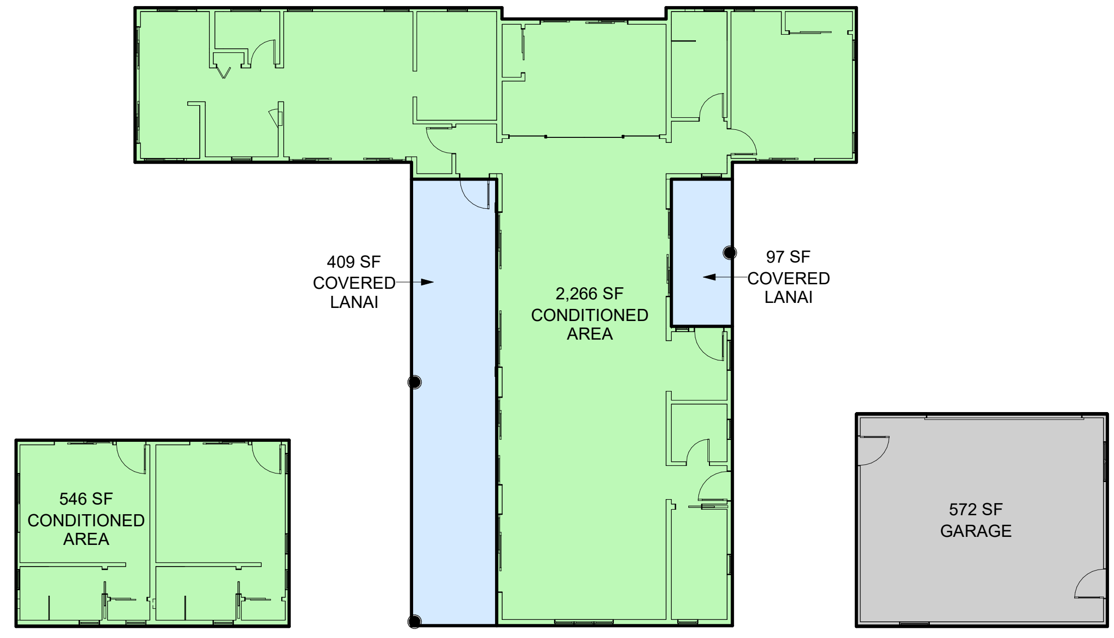
2 AREA CALCULATIONS SCALE: 1" = 10'-0"
