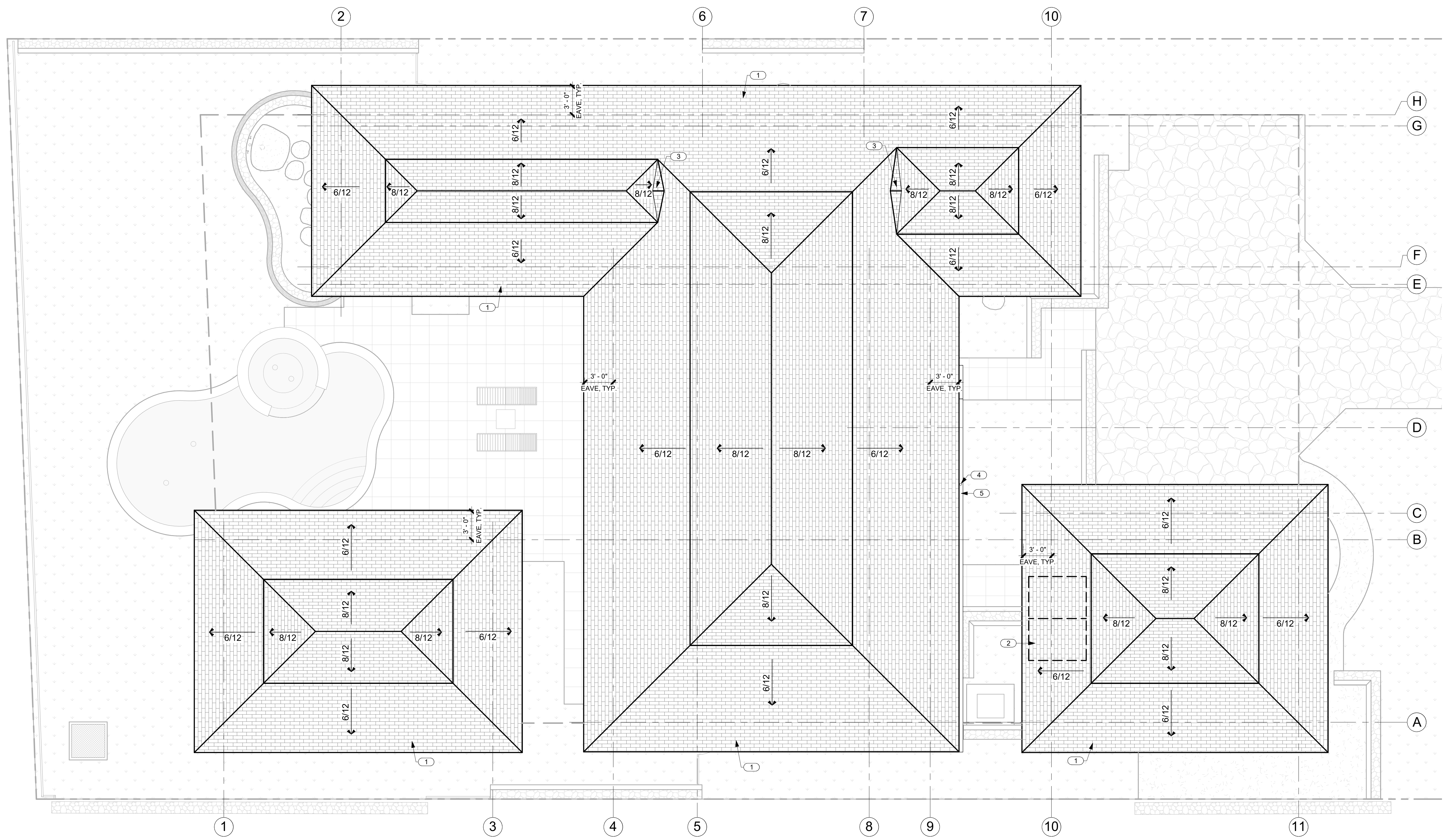
1 ROOF PLAN A2.5 SCALE: 3/16" = 1'-0"
