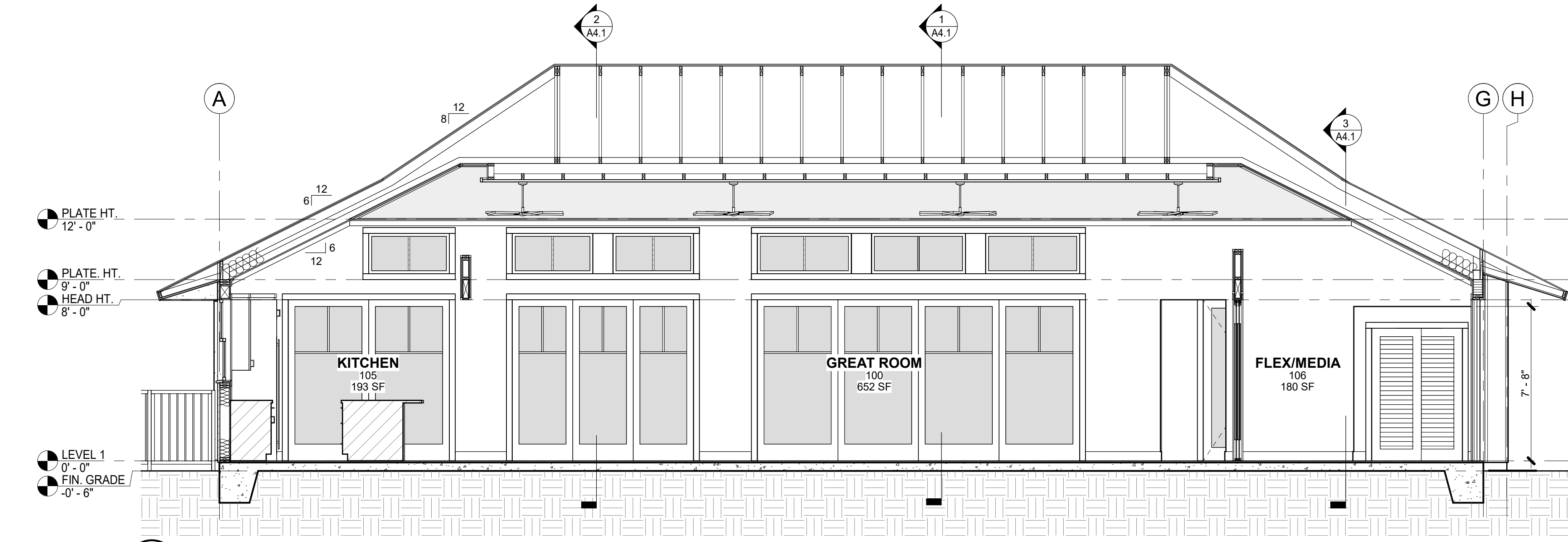
2 SECTION THRU GREAT ROOM LOOKING WEST SCALE: 1/4" = 1'-0"
