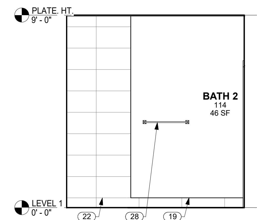
14 SOUTH WALL BATH 114 A7.0 SCALE: 3/8" = 1'-0"
