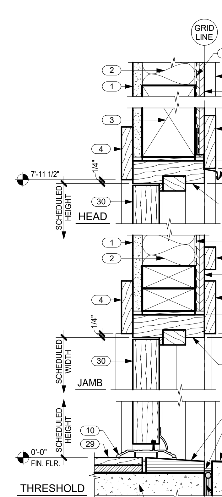
9 TYP. HINGED DOOR DETAILS IN SIDING A6.1 SCALE: 3" = 1'-0"
