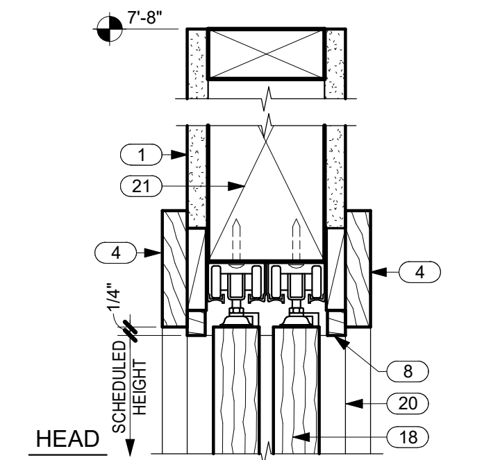
4 TYP. RECESSED SLIDING DOOR TRACK A6.1 SCALE: 3" = 1'-0"
