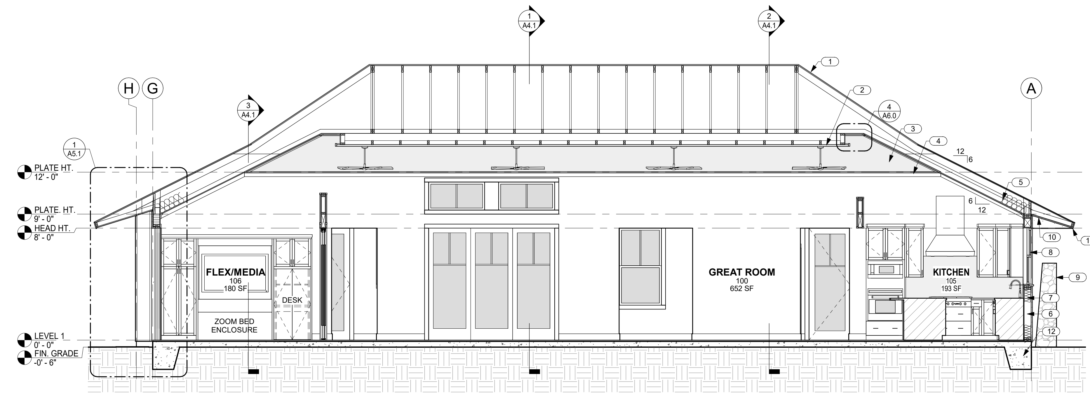
1 SECTION THRU GREAT ROOM LOOKING EAST SCALE: 1/4" = 1'-0"
