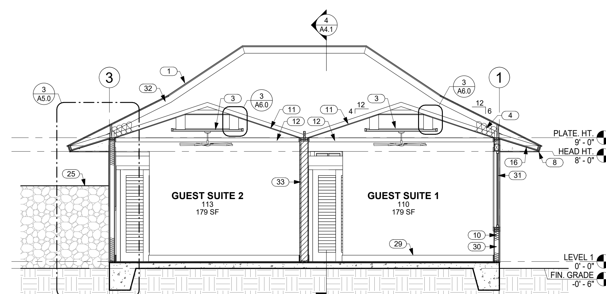
5 SECTION THRU GUEST SUITES 1 AND 2 LOOKING NORTH
