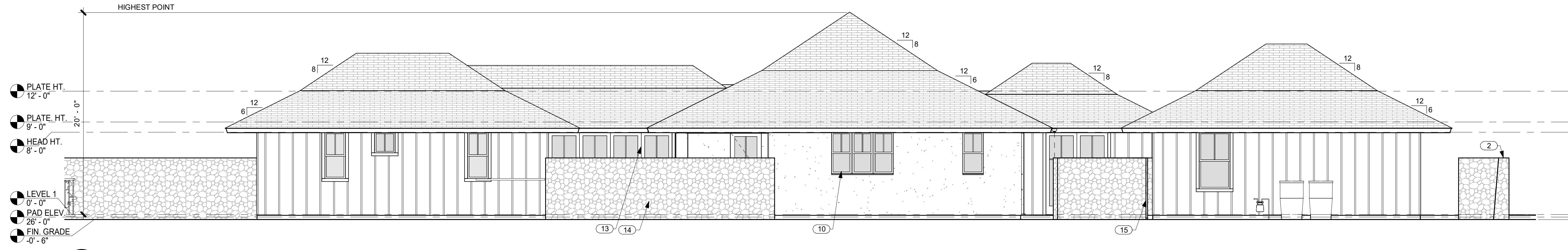
1 EAST ELEVATION A3.0 SCALE: 3/16" = 1'-0"
