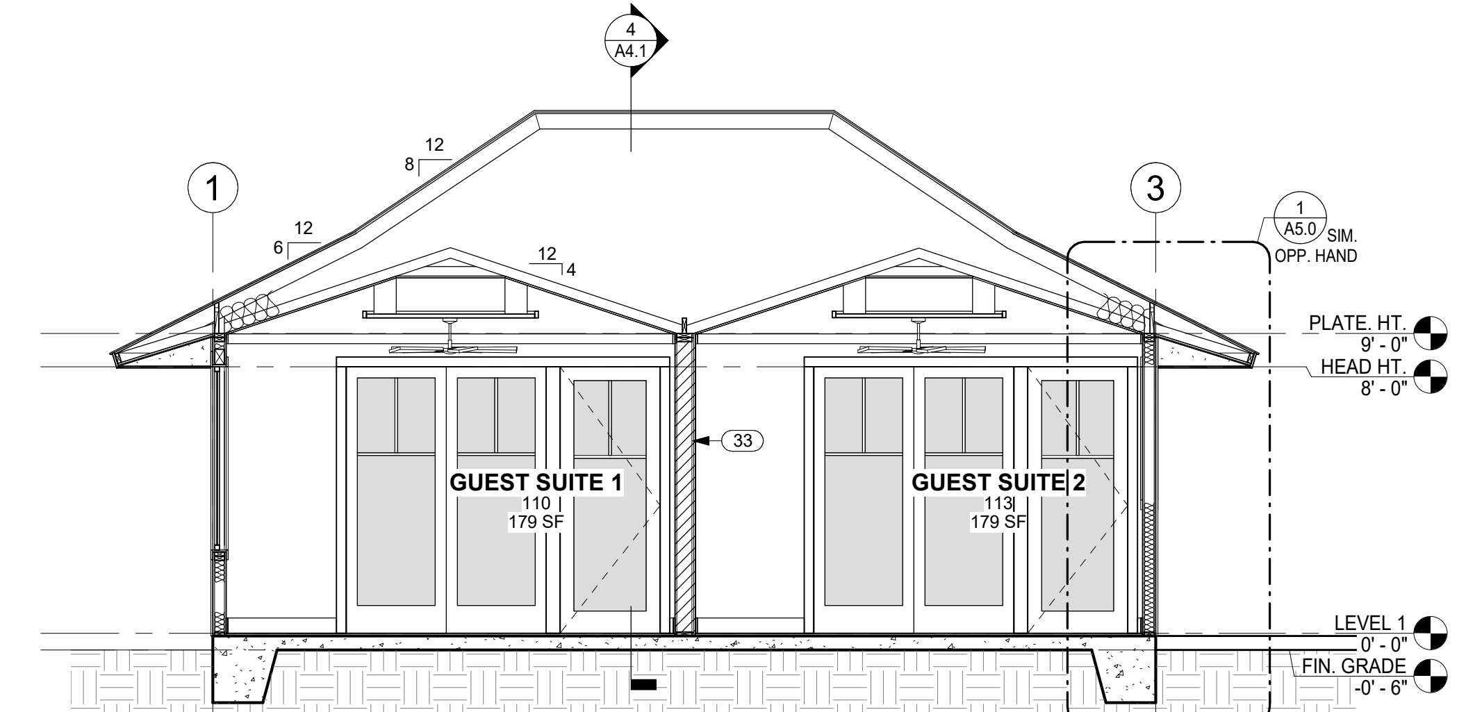
6 SECTION THRU GUEST SUITES 1 AND 2 LOOKING SOUTH
