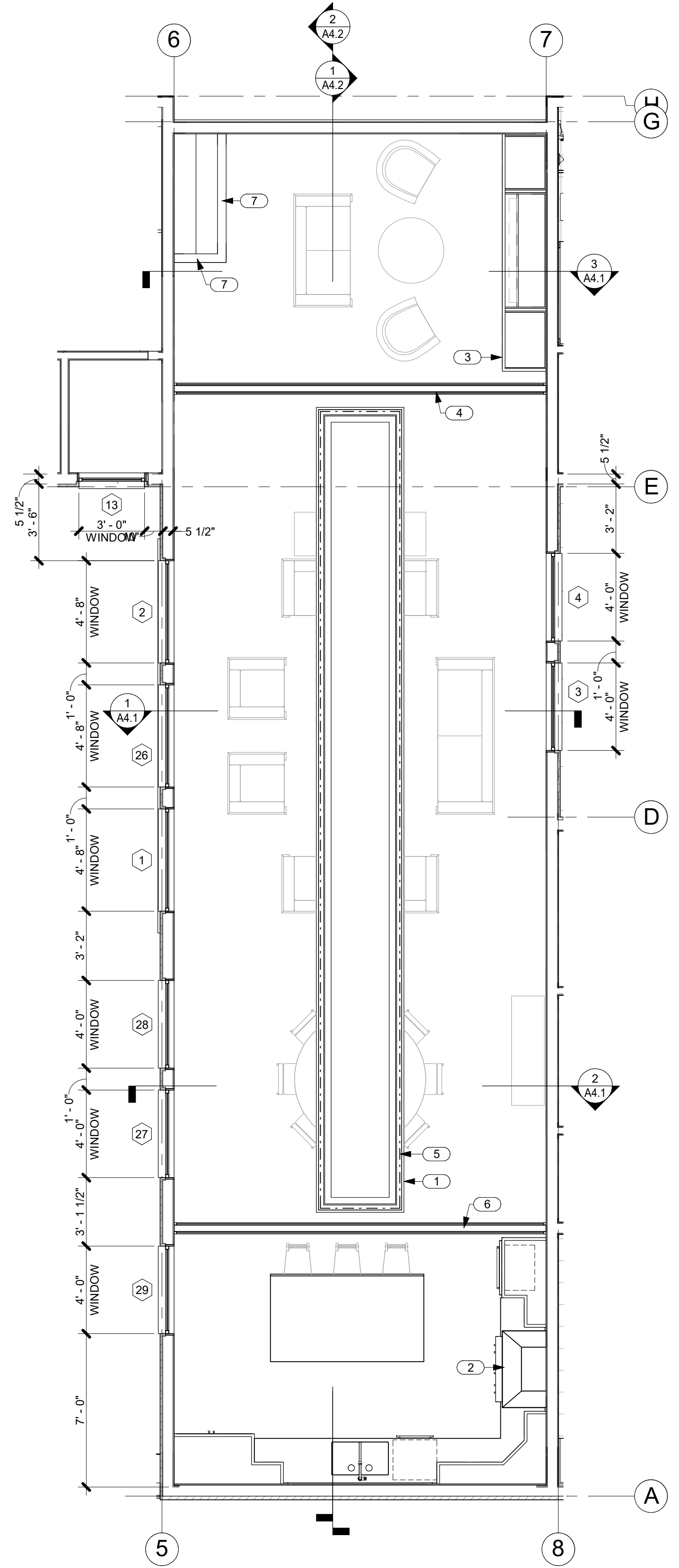
1 CLERESTORY PLAN SCALE: 1/4" = 1'-0"
