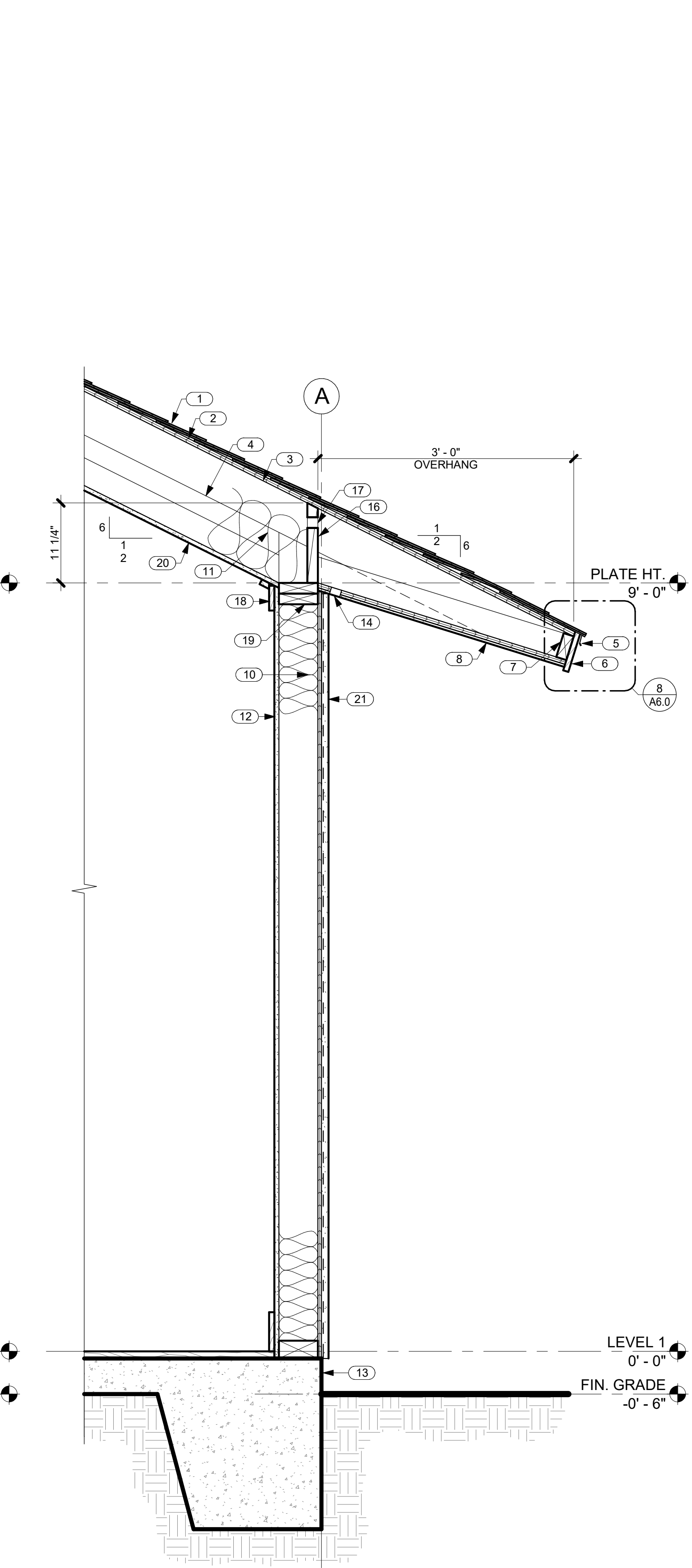
4 SECTION THRU NORTH WALL OF GREAT ROOM LOOKING WEST A5.0 SCALE: 1" = 1'-0"
