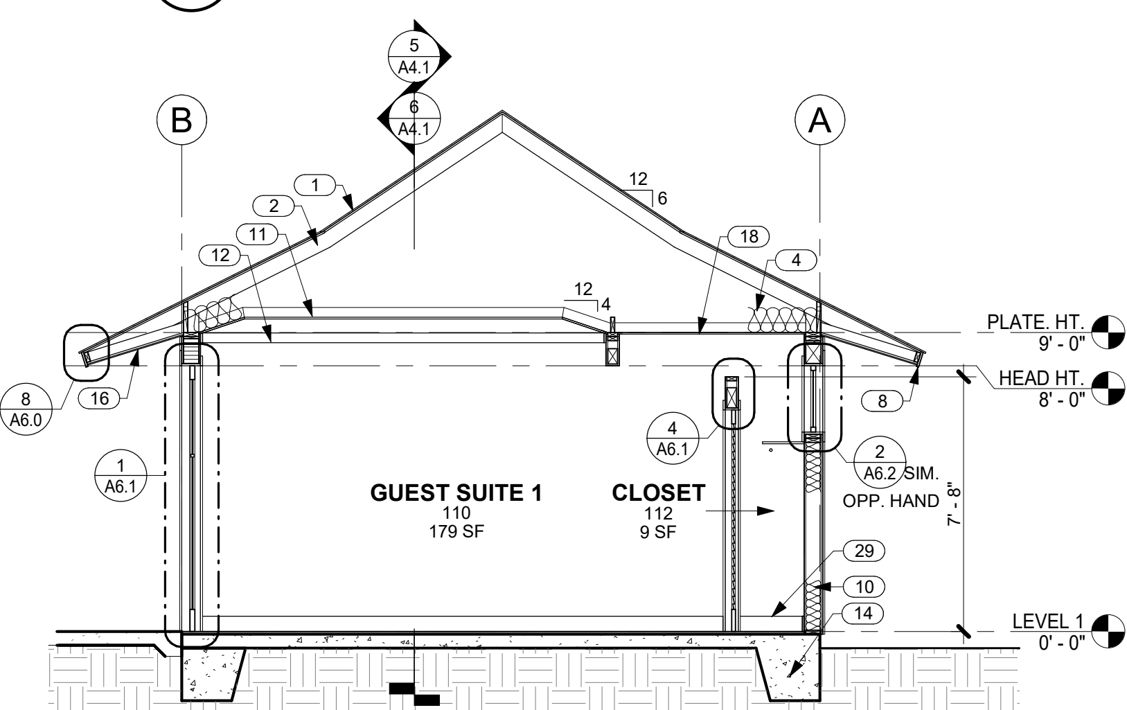
4 SECTION THRU GUEST SUITE 1 LOOKING EAST
