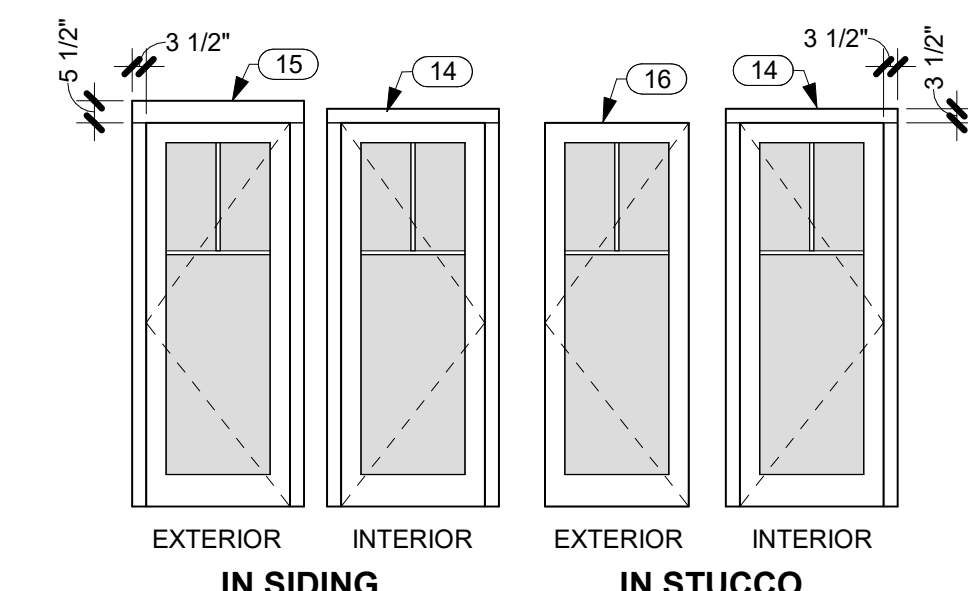
6 TYPICAL DOOR ELEVATIONS A6.1 SCALE: 1/4" = 1'-0" NOTE: NO INTERIOR CASING @ TILE WALLS.
